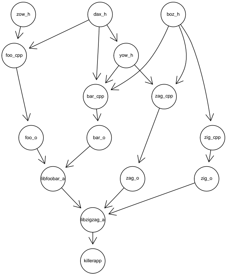
Figure 2: File dependency digraph example from Boost library.
