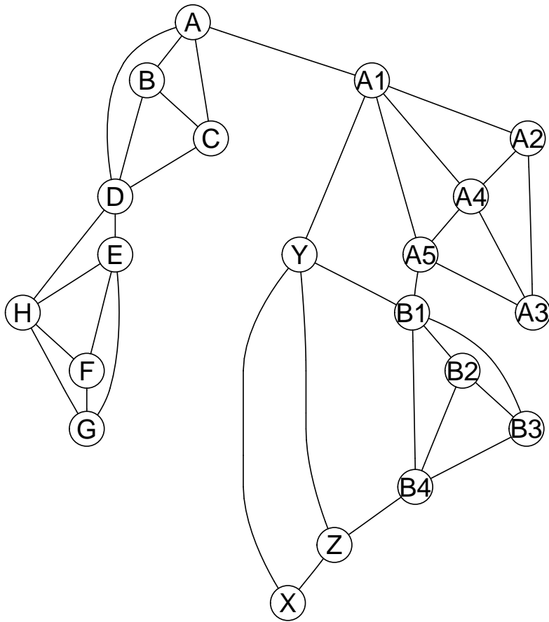
Figure 9: Example on incremental components: a graph connecting coex and hcs.
