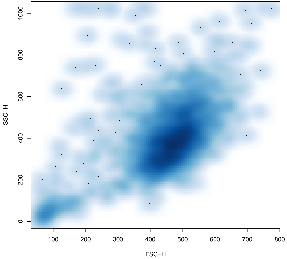
Figure 4: Smooth scatter plots.
