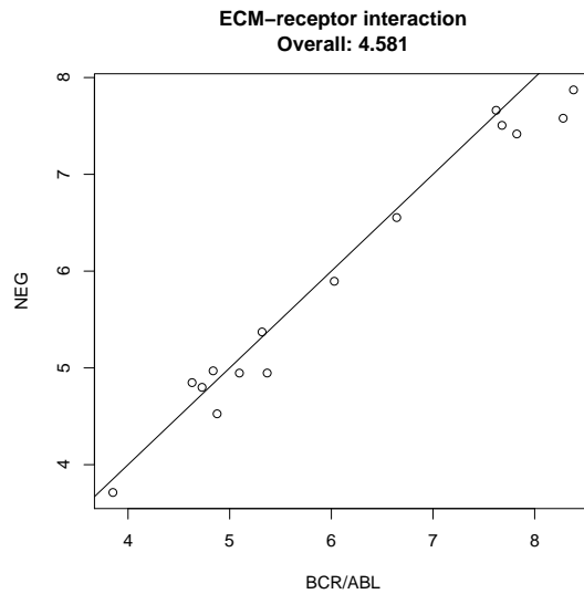
Figure 6: The per category mnpplot for pathways that are deemed to be differentially expressed using a permutation approach.
