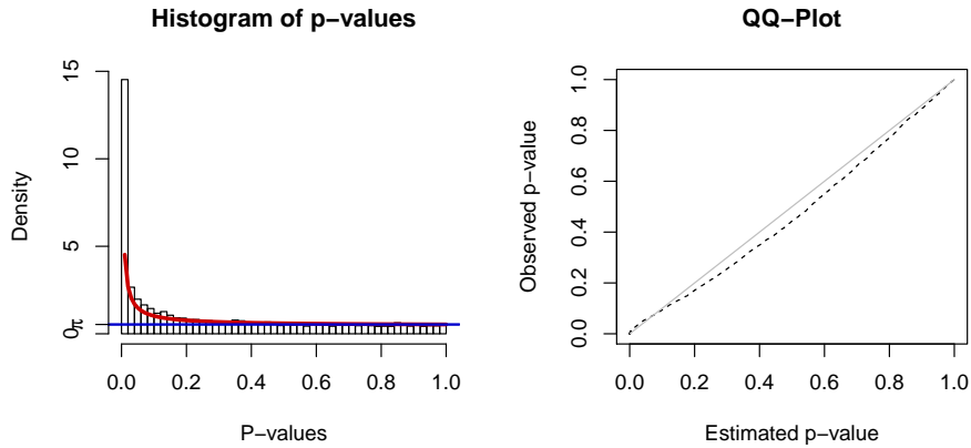
Figure 7: Histogram of p-values, overlaid by the fitted BUM model in red and the \pi -upper bound displayed as a blue line. The right plot shows a quantile-quantile plot, in which the estimated p-values from the model fit deviate slightly from the observed p-values.
