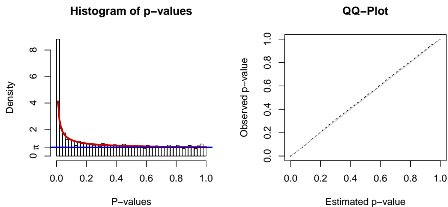
Figure 3: Histogram of p-values, overlaid by the fitted BUM model coloured in red and the \pi -upper bound displayed as a blue line. The right plot shows a quantile-quantile plot, indicating a nice fit of the BUM model to the p-value distribution.
