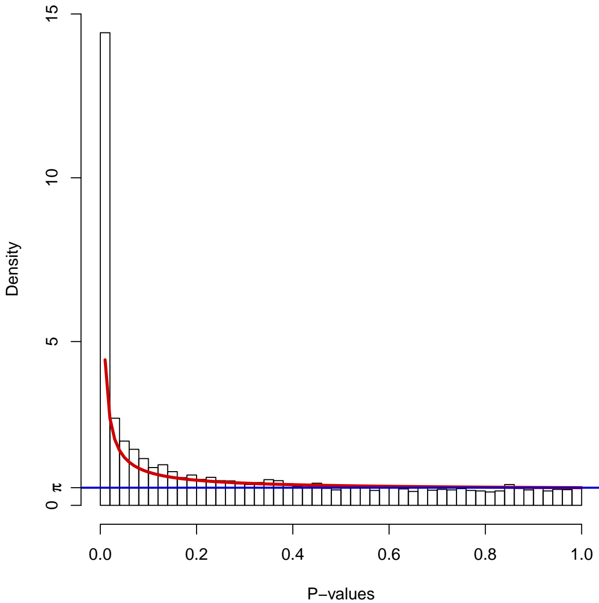
Histogram of p-values
