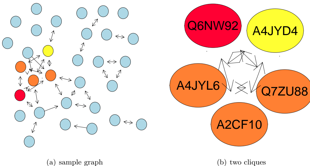
Figure 3: Two cliques of size 4 found in the example network, colored with yellow (A4YJD4) and red (Q6NW92) individually. The two cliques share three common nodes, whose color is orange due to blending.
