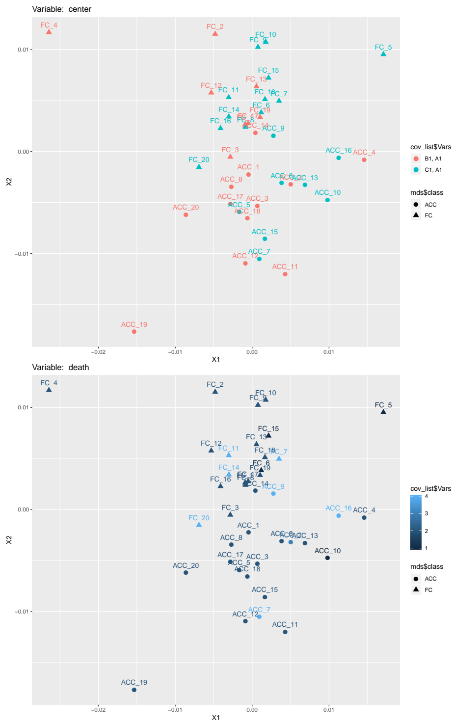
Figure 7: MultiDimensional Scaling plot
