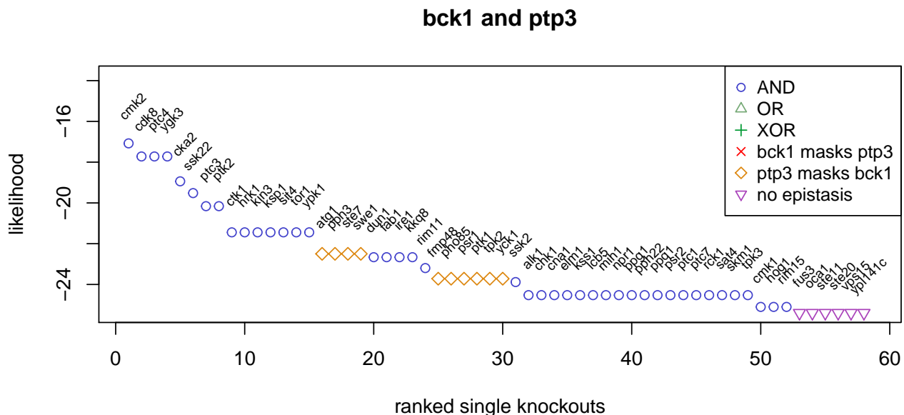
Figure 7: Results for one double knock-out of the van Wageningen data set. See ?plot.epiScreen for further parameters.
