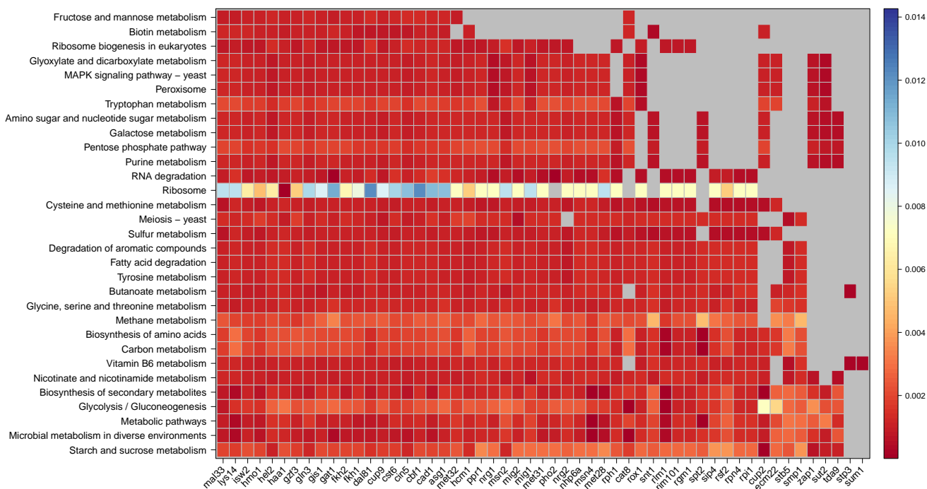
Figure 17: Effect reporter KEGG pathway enrichment (Sameith). Colors refer to false discovery rates. NAs are colored in grey.
