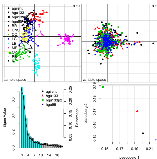
Figure 2: The MCI plot of NCI-60 data
