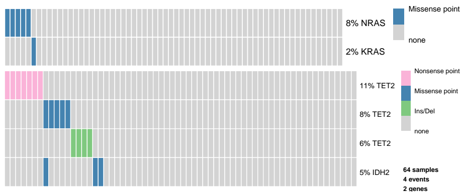
Figure 7: anoncoprint output to show the perfect (hard) exclusivity among NRAS/KRAS mutations in aCML on top, and the softy-one among TET2 and IDH2 alterations
